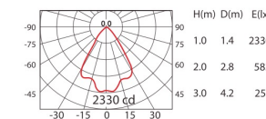
CoB 3800lm 900mA WW 70°
