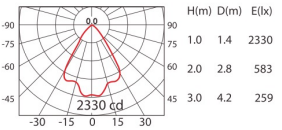
CoB 3800lm 900mA WW 70°
