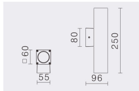
OBA-132S (SHARP) CoB: 1300lm 13W(350mA,37V) AC 120-240V
