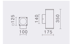
OBA-136S (CITIZEN) CoB: 3100lm 25.5W(700mA,36V) AC 120-240V
