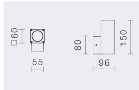
OBA-112S (SHARP) CoB: 1300lm 13W(350mA,37V) AC 100-240V
